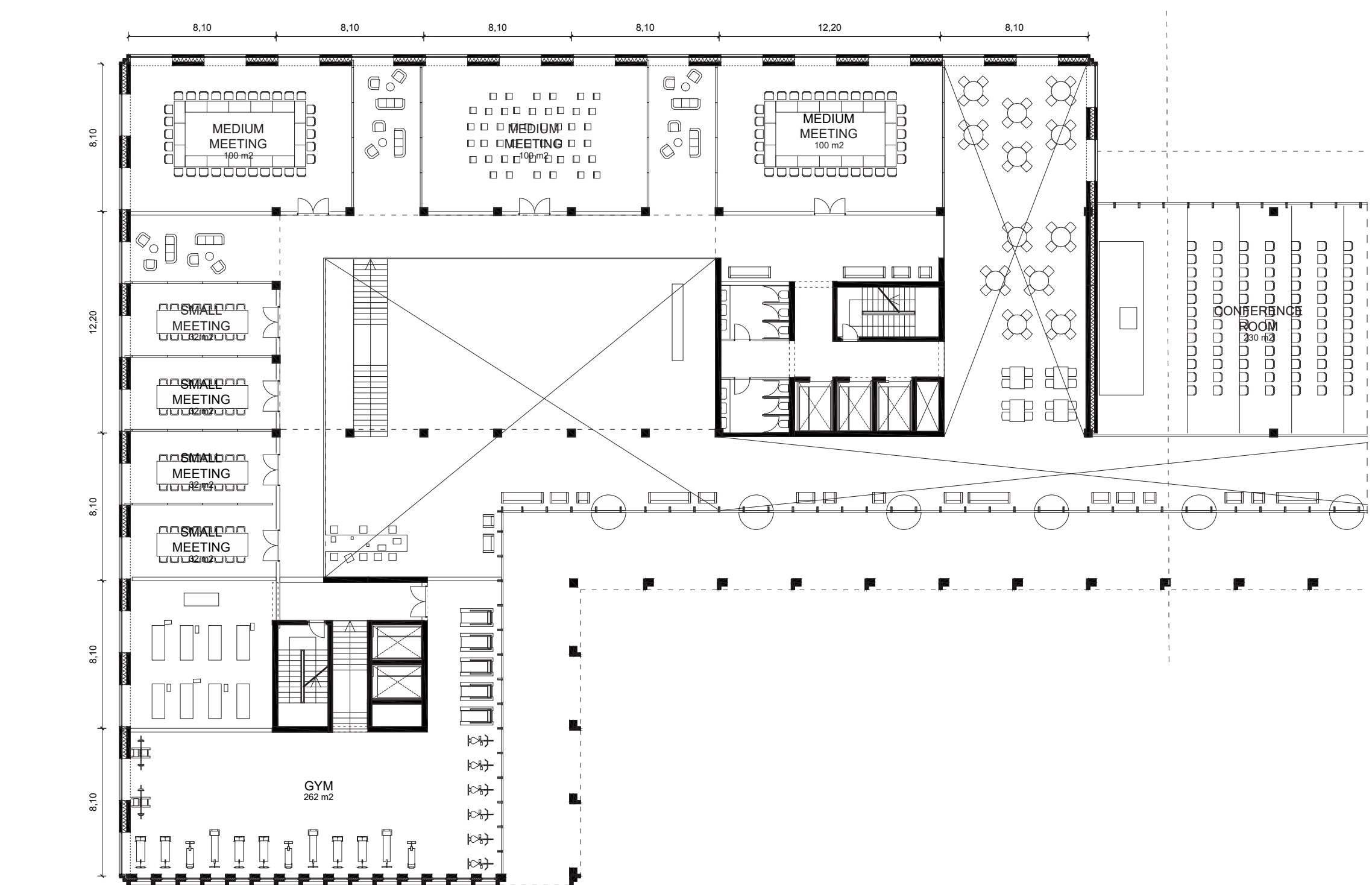
Floorplan, level +1 1:250
