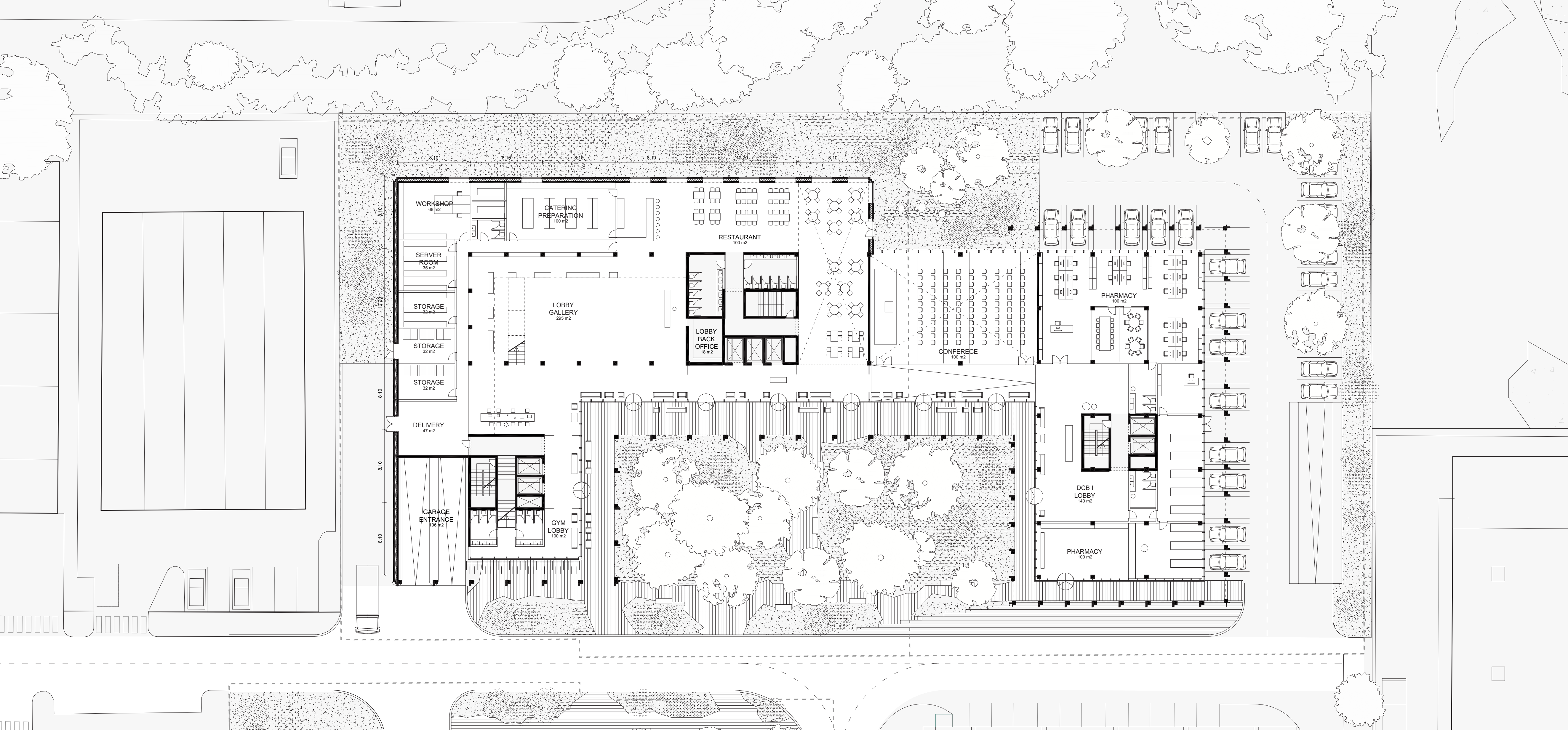
Floorplan, level 0 1:250
