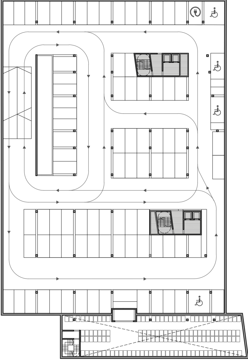
DBII basement floor 1:250
