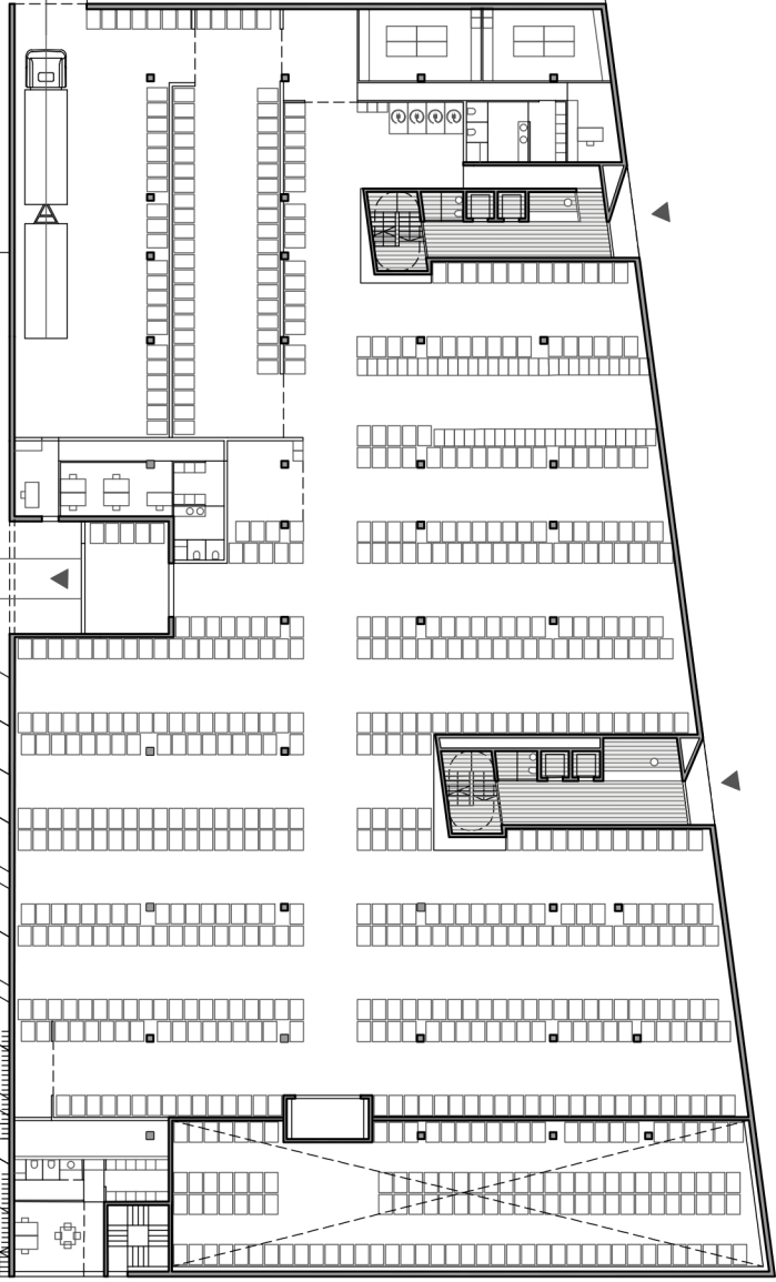
DBII ground floor 1:250
